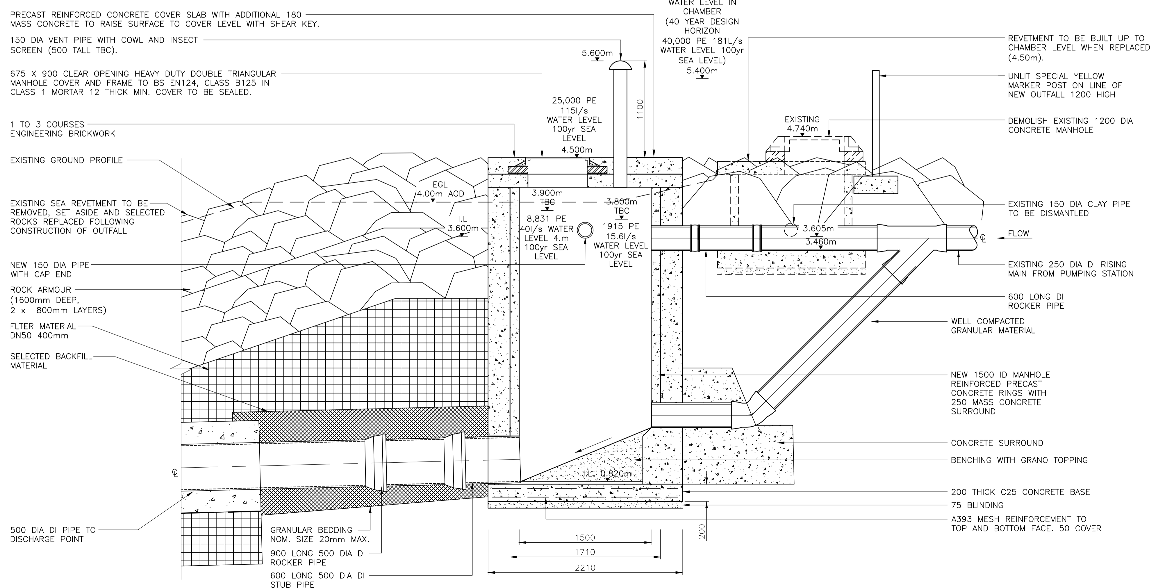
CHAMBER SECTION A-A SCALE 1:25
