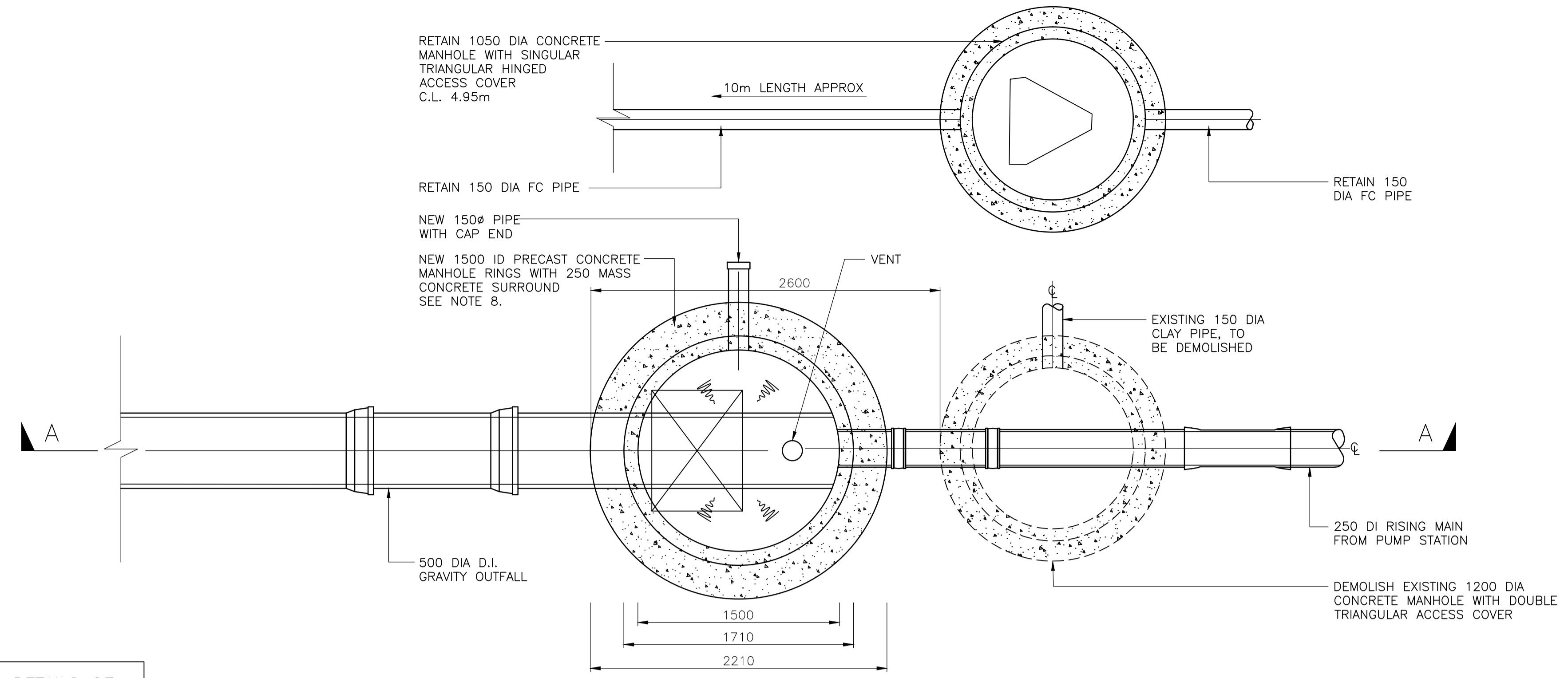
CHAMBER PLAN VIEW SCALE 1:25
