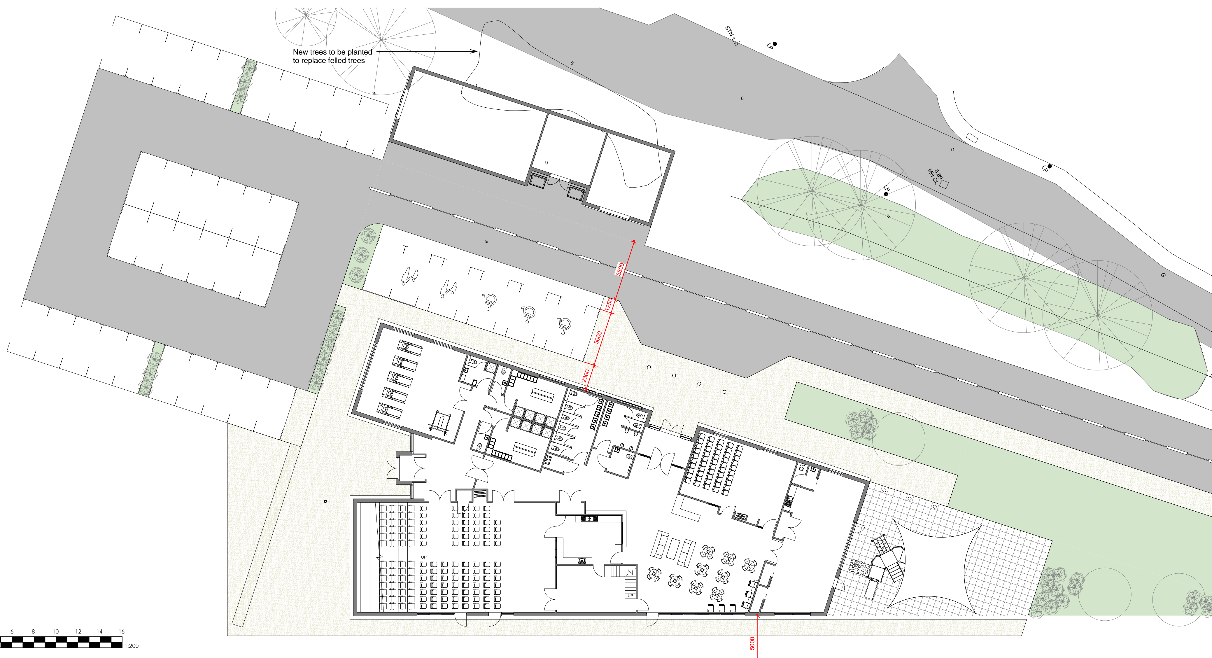
1 Proposed Site Plan 1:200
