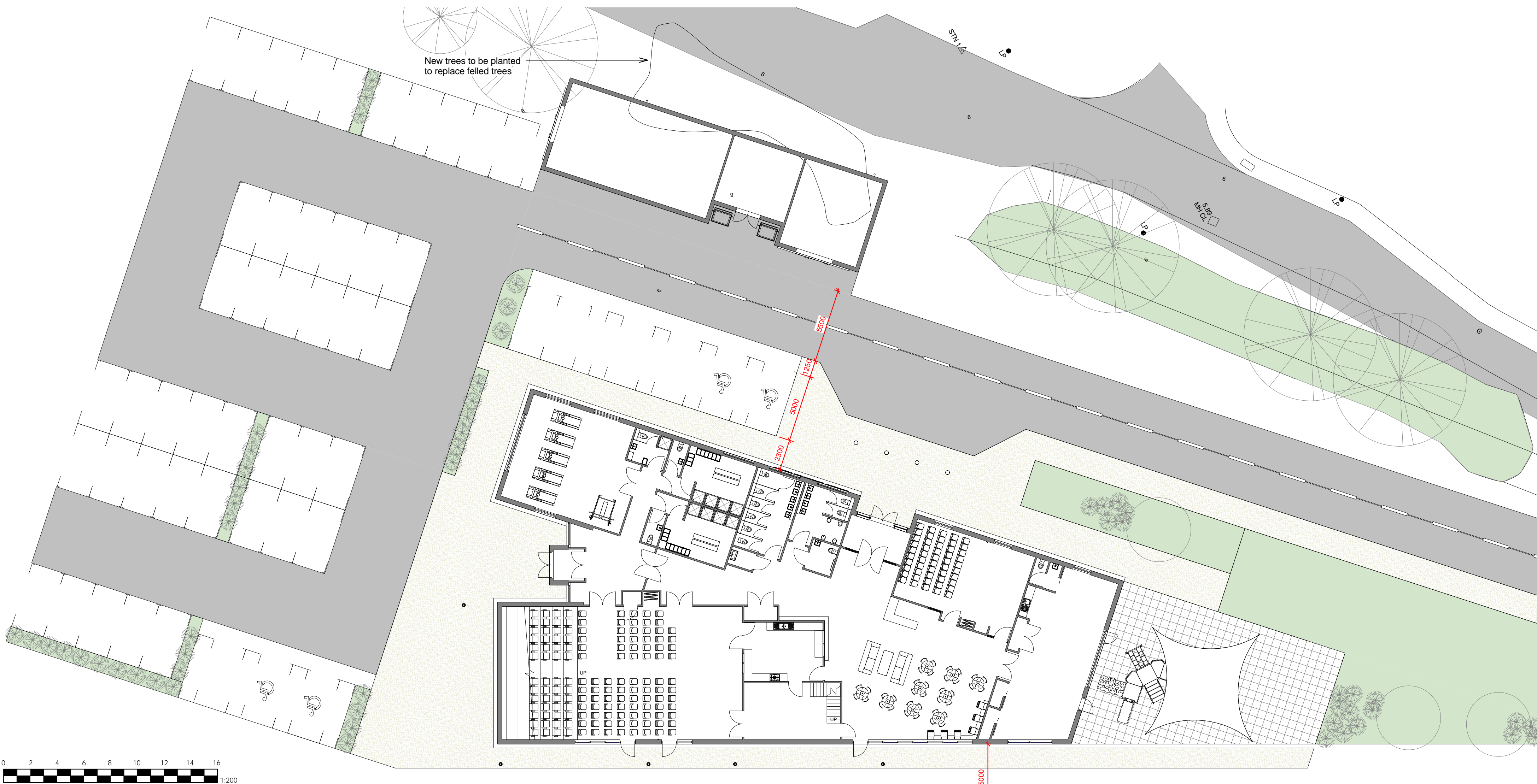
1 Proposed Site Plan 1 : 200
