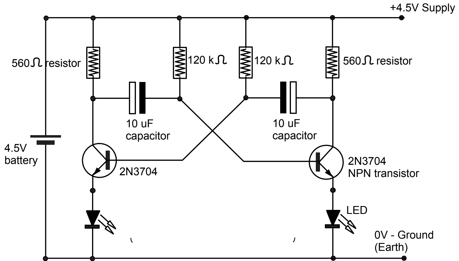
Astable flasher LED circuit
